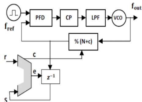
Fig. 1 .b . Block diagram of a classical fractional-N PLL [1]
